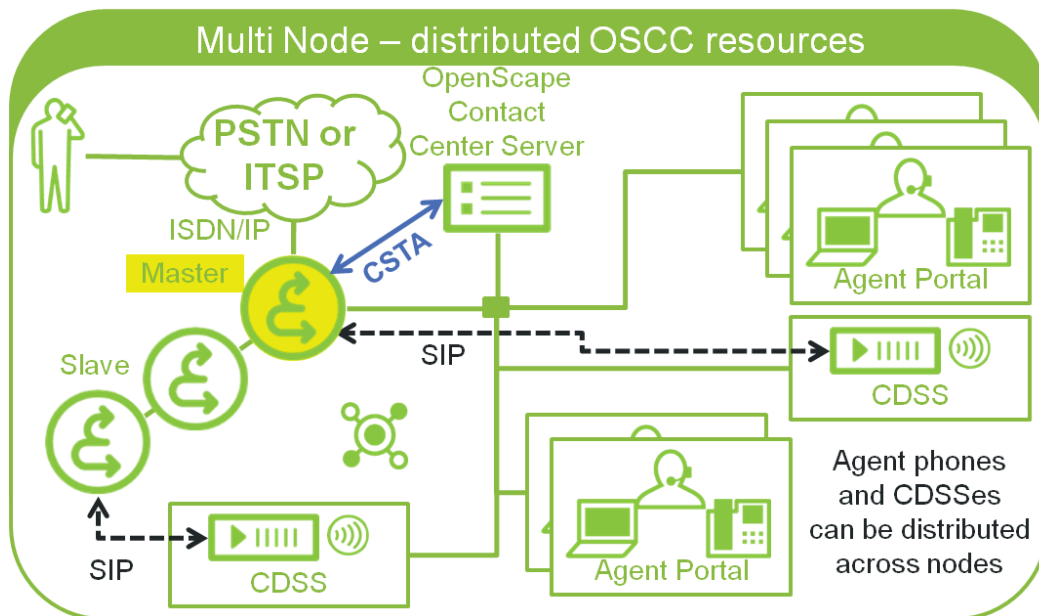
Figure 39 Example: OSCC connected to master node with distributed resources
