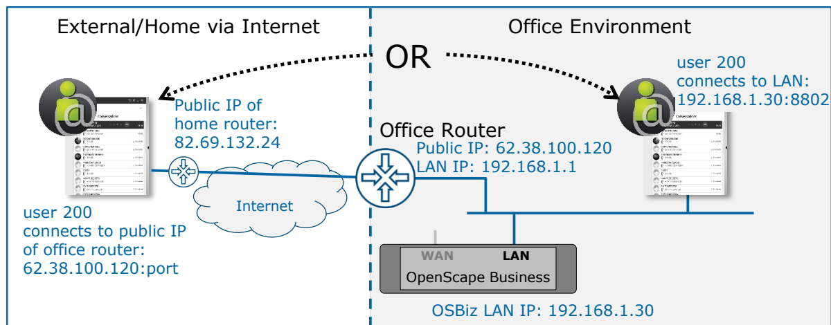
Figure 20 myPortal @work client in the office and at home via public Internet
