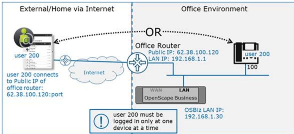
Figure 21 myPortal @work client user at home via public Internet as Deskshare user in the office
