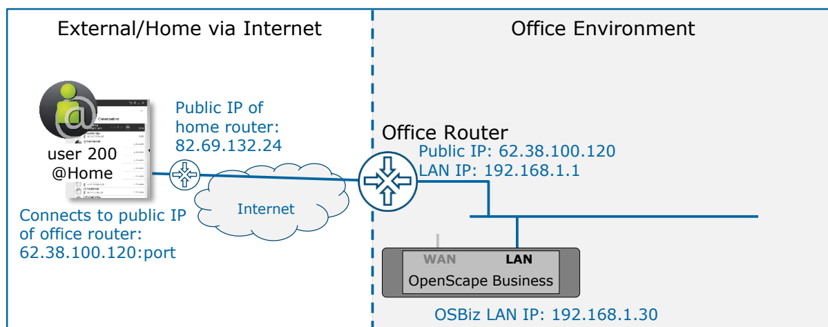
Figure 19 myPortal @work user at home via Internet connection
