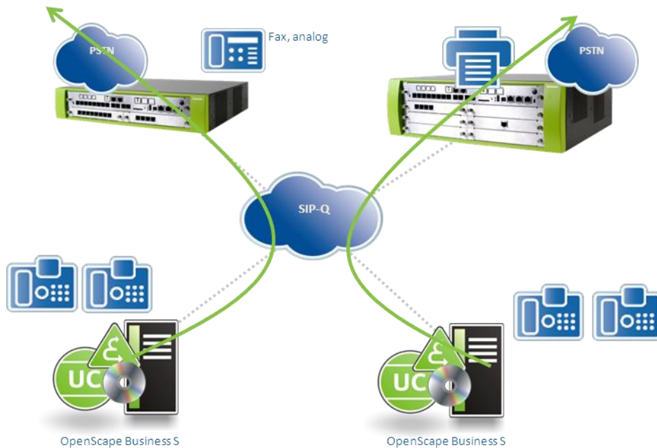
Figure 48 Networking OpenScape Business X1/X3/X5/X8 with OpenScape Business S (single gateway)
