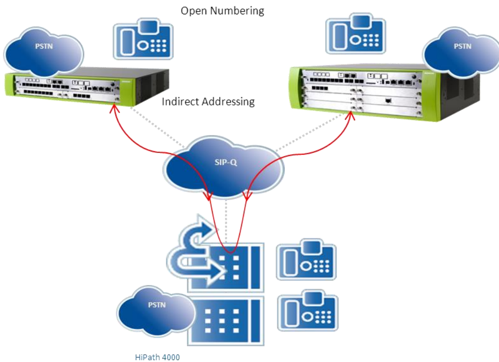
Figure 51 Network Connection with OpenScape 4000 (all connections are routed via OpenScape 4000)
