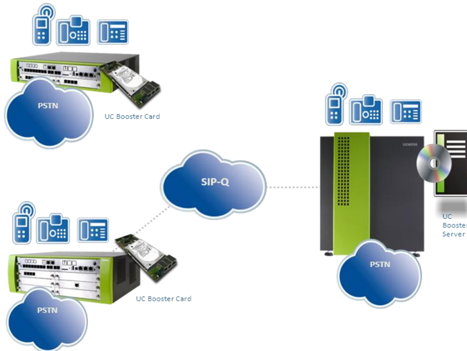
Figure 47 Networking several OpenScape Business X1/X3/X5/X8
