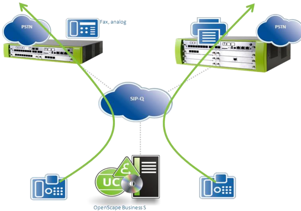
Figure 49 Networking OpenScape Business X1/X3/X5/X8 with OpenScape Business S (multi gateway)
