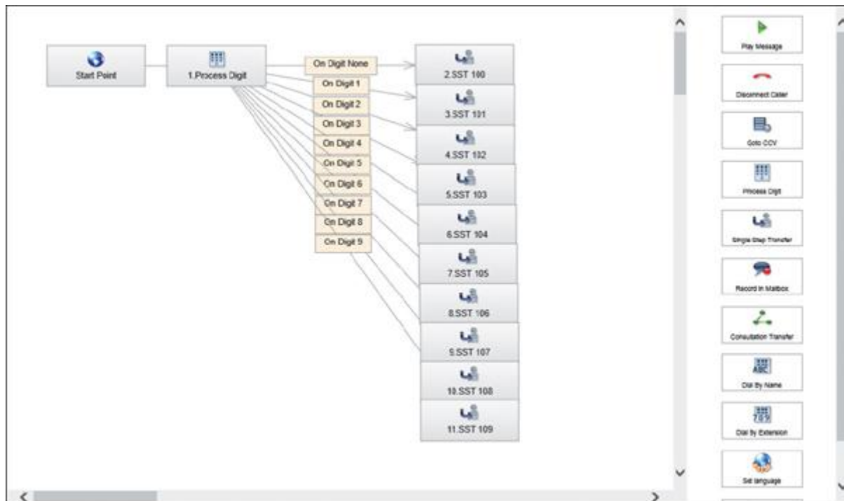
Figure 37 UC Suite – Auto Attendant Setup
