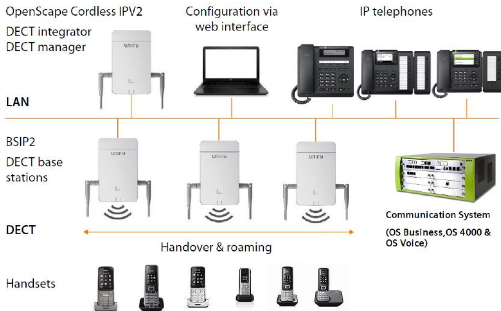
Figure 34 Cordless IP – Connection overview
