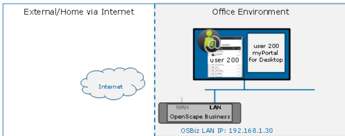
Figure 22 myPortal for Desktop together with myPortal @work
