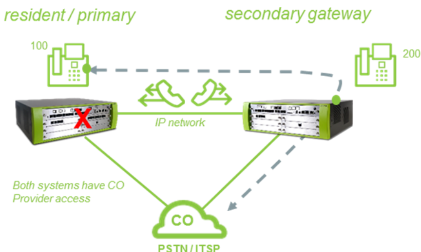
Figure 56 IP Telephony Redundancy – Trunk Line Connection in Primary and Secondary System
