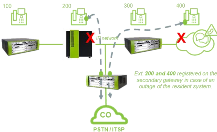
Figure 57 Multiple primary systems, trunk line connection only in the secondary system
